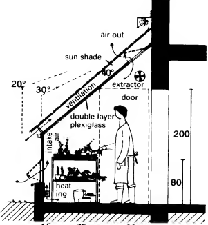
⑩ Lean-to greenhouse
